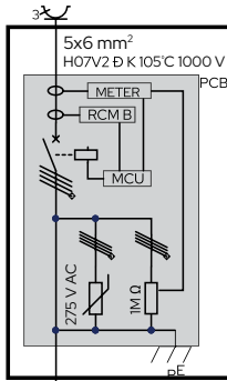
Charging module Type 2 socket with RCM B 6 mA DC
