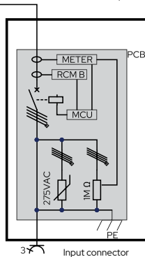
Charging module Type 2 socket with RCM B 6 mA DC
