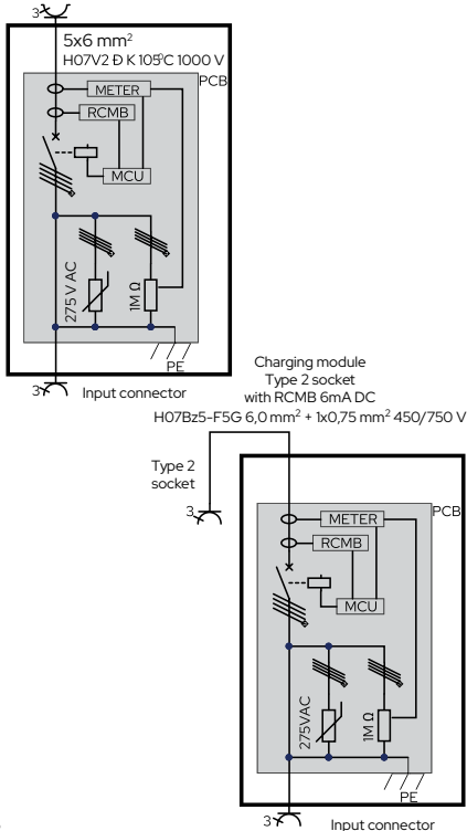
Charging module Type 2 socket with RCMB 6 mA DC
