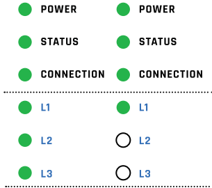
Fig. 27: Three-Phase and Single-Phase Connection Indication
