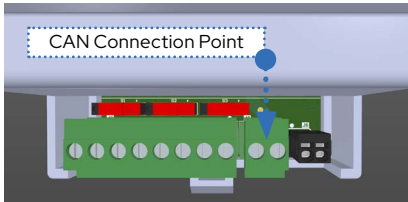
Fig. 14: Connection Point for CAN Wires to EEG 3.0
