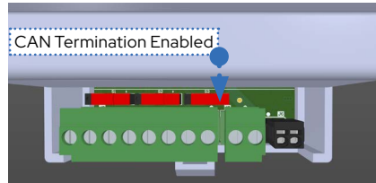
Fig. 15: CAN Connection Termination Enabled (switch in right position)
