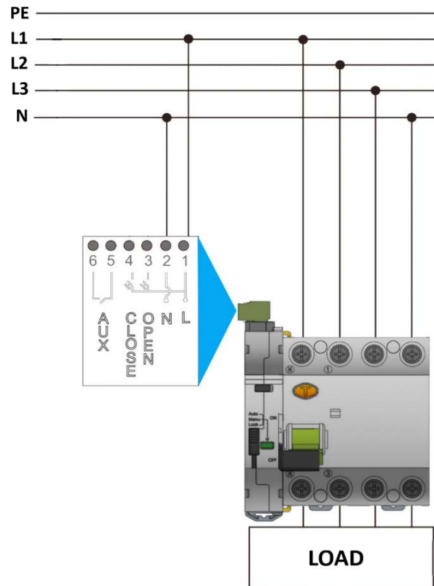
Fig. 14: Instructions for connecting RCD B with an automatic reclosing device to the power supply.
