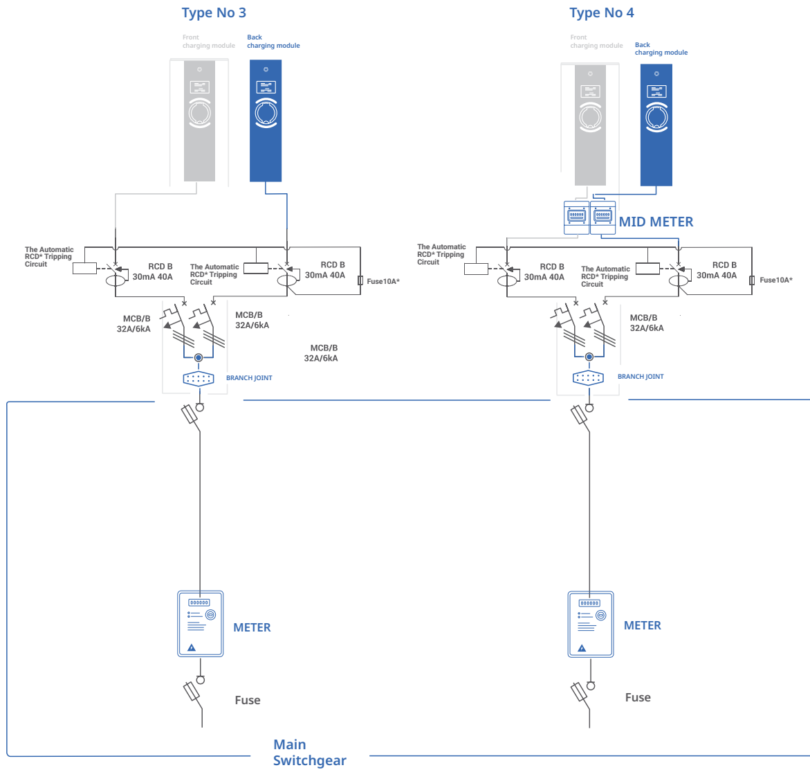
Fig. 17: Connection types part 2/3
