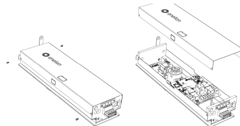
Fig. 77: Opening the Enelion VERTICA module.
