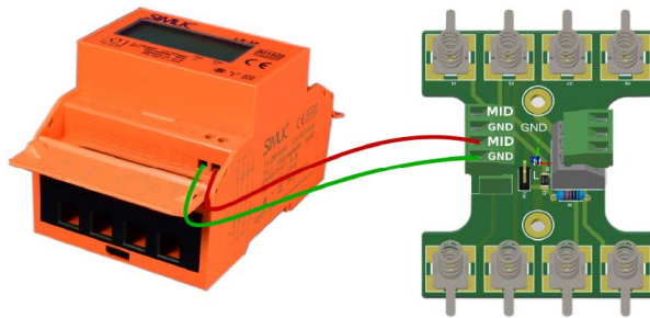
Fig. 47: Wiring diagram for MID meter communication wires for a Enelion VERTICA pole equipped with a Enelion VERTICAN module.
