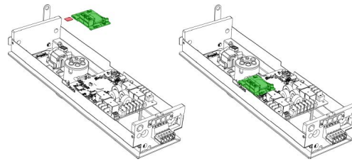
Fig. 69: Installing Enelion Bridge in the Enelion VERTICA Module.
