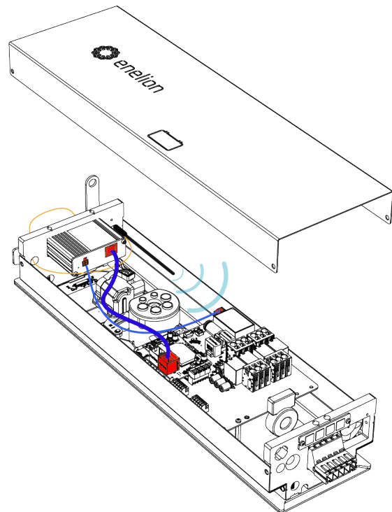
Fig. 80: Properly mounted LTE module.
