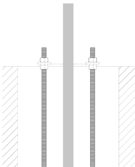
Fig. 30: Details of placing the upper base plate in the excavation
