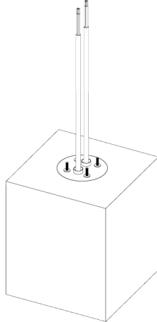
Fig. 24: Properly constructed foundation using the prefabricated element.
