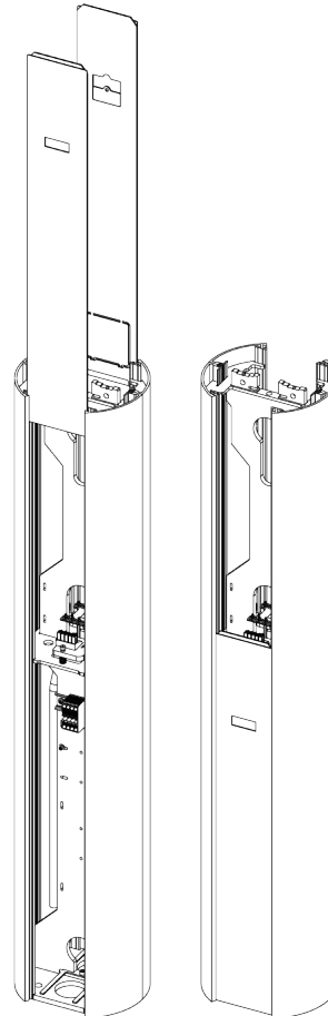
Fig. 67: Reverse of the Enelion VERTICA Pole after mounting the Enelion VERTICA Splitter with the MID meter present.
