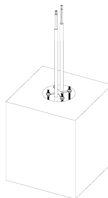
Fig. 31: Foundation set correctly placed in the excavation
