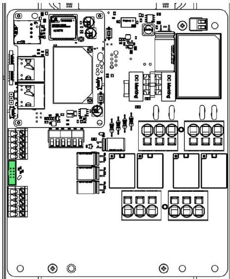
Fig. 75: Communication connector of the Enelion RCMB add-on.
