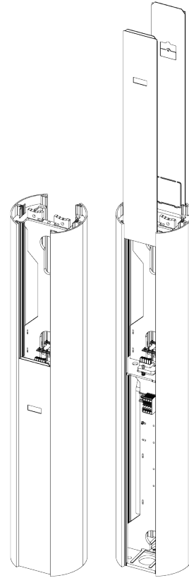
Fig. 36: Sliding the lower masking panels out of the Enelion VERTICA Pole.
