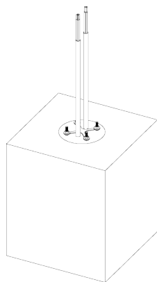
Fig. 33: Correctly cast foundation set.
