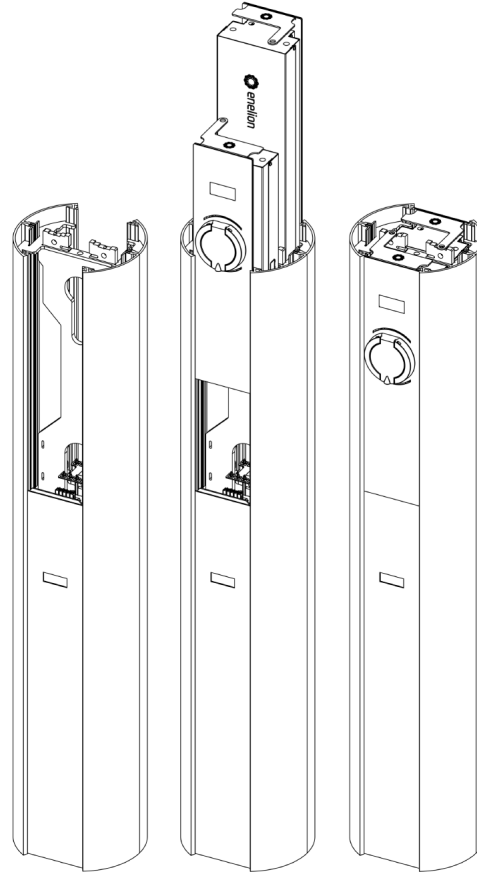
Fig. 13: Assembly of Enelion VERTICA Modules
