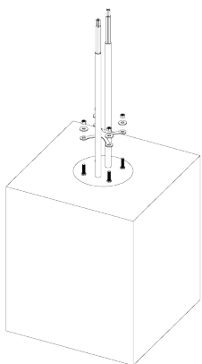
Fig. 34: Removing of the upper base plate from the foundation set.
