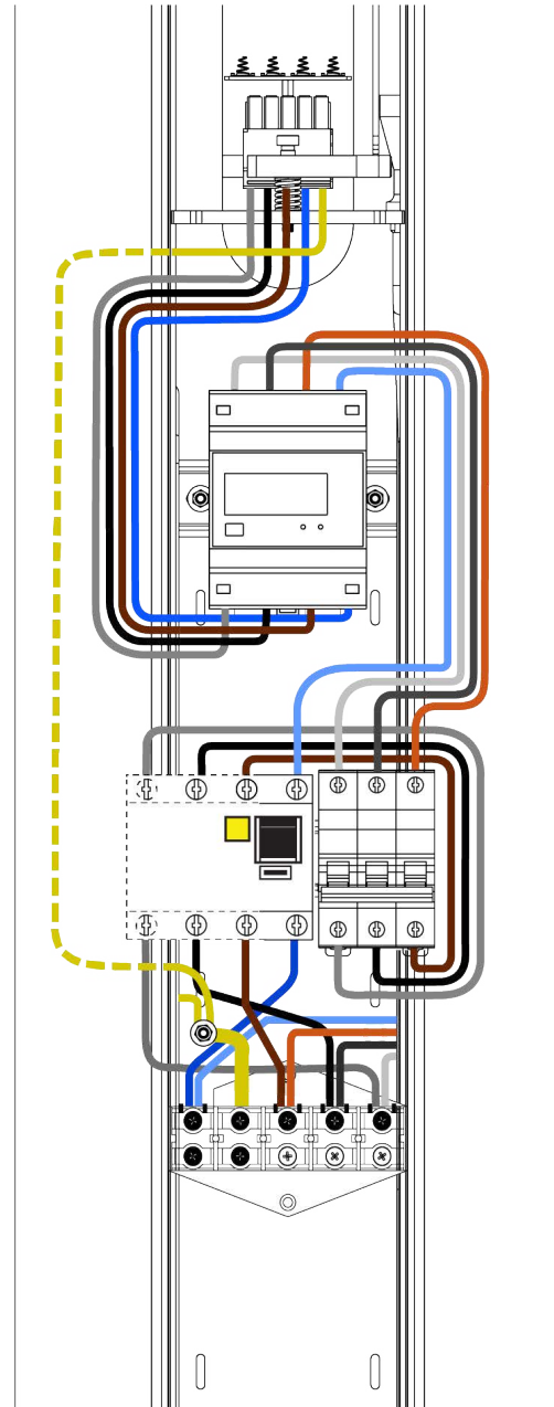
Fig. 65: Obverse of the Enelion VERTICA Pole after mounting the Enelion VERTICA Splitter with the MID meter present.
