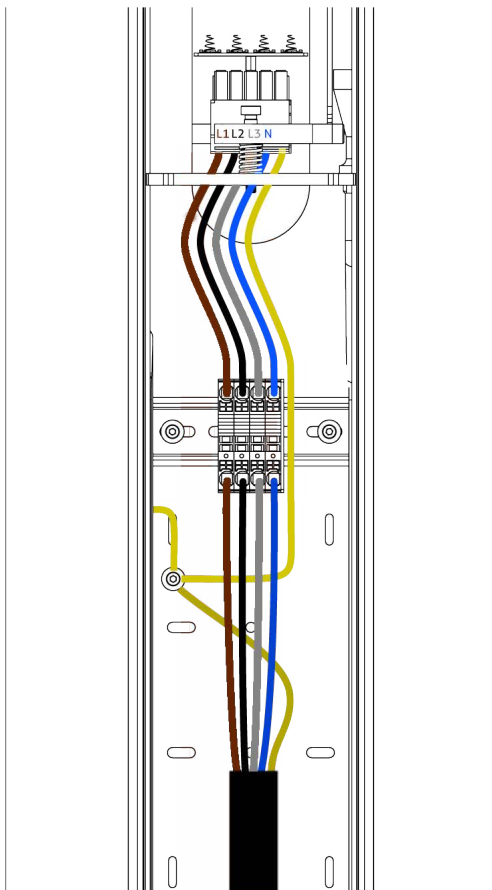
Fig. 41: Example Enelion VERTICA Pole connection.
