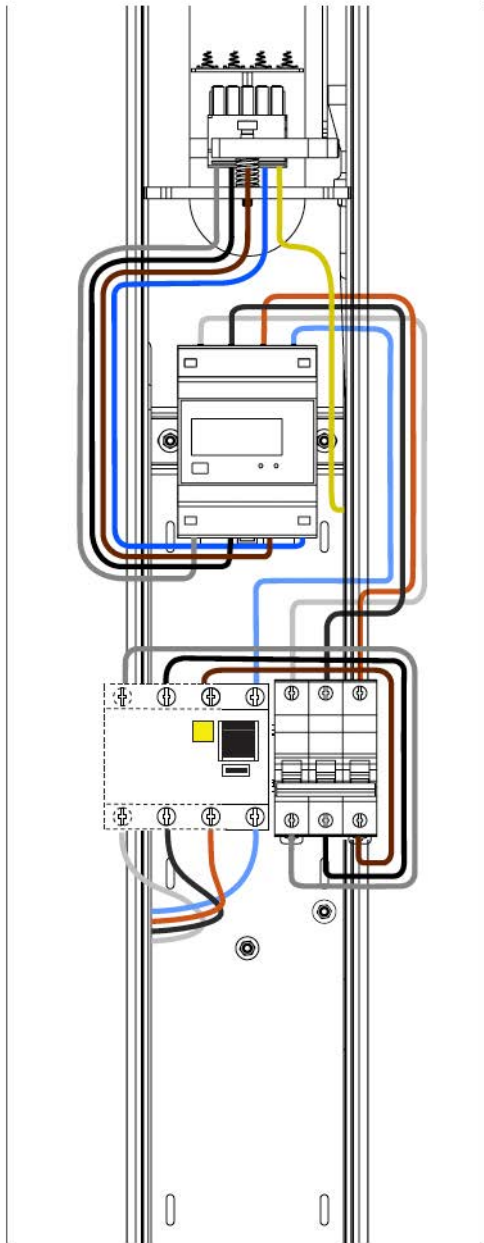
Fig. 66: Reverse of the Enelion VERTICA Pole after mounting the Enelion VERTICA Splitter with the MID meter present.
