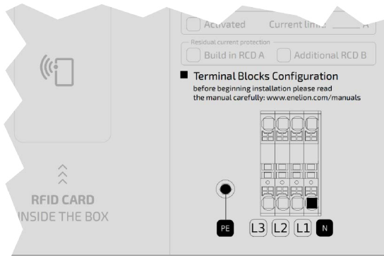
Fig. 40: Sample part of a product label
