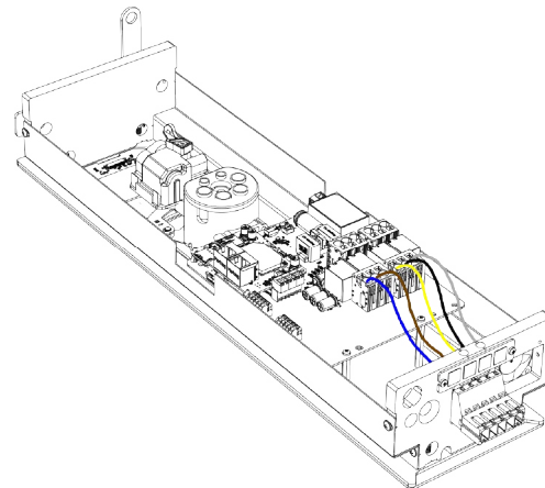
Fig. 73: The charging controller power connector on the Enelion VERTICA Module.
