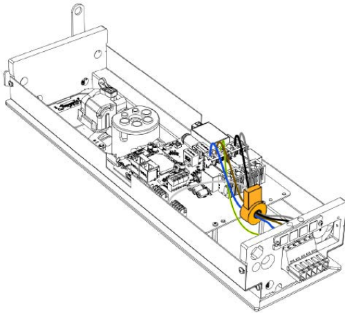
Fig. 74: Enelion VERTICA module during installation of Enelion RCMB.
