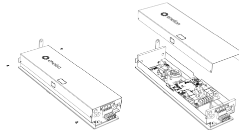
Fig. 72: Opening the Enelion VERTICA Module.
