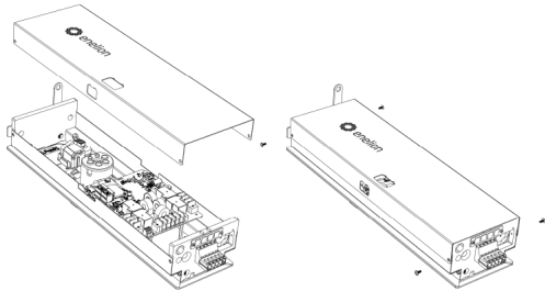
Fig. 71: Closing the Enelion VERTICA Module.
