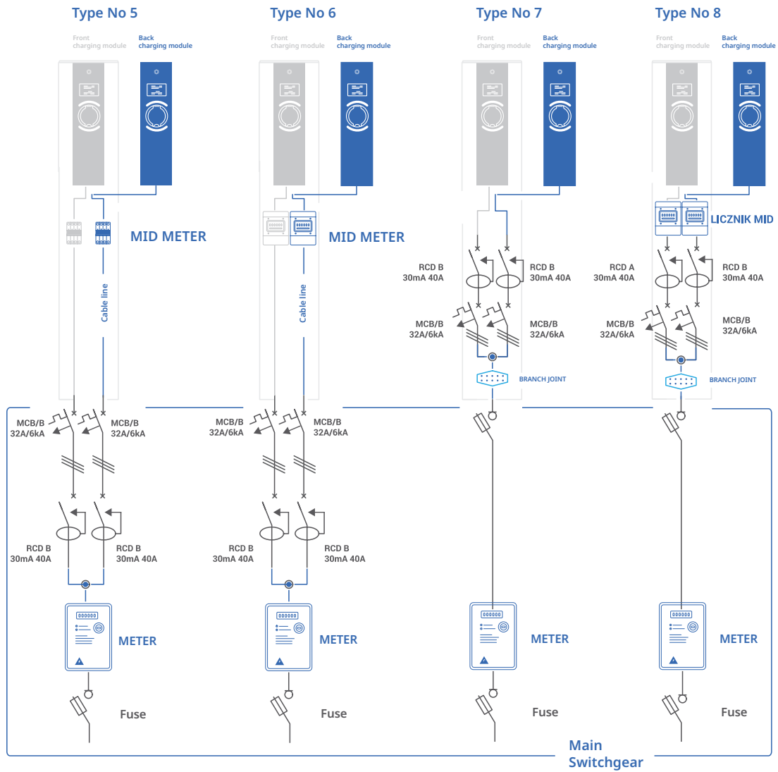
Fig. 18: Connection types part 3/3
