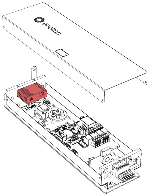
Fig. 78: Mounting the LTE module.
