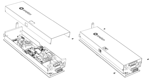
Fig. 68: Opening the Enelion VERTICA Module.
