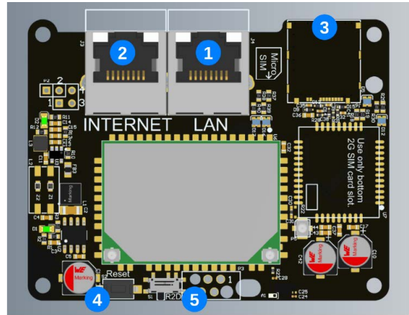
Fig. 54: The Enelion Bridge module
