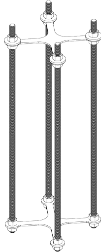
Fig. 27: Enelion foundation set.
