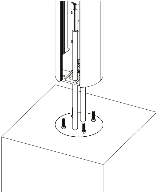
Fig. 37: Mounting Enelion VERTICA Pole on the foundation.
