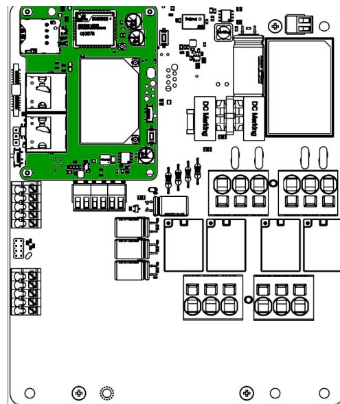
Fig. 70: Enelion Bridge attached to the Enelion VERTICA Module.
