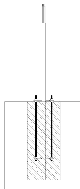
Fig. 32: Cross-section of the foundation set cast in the concrete
