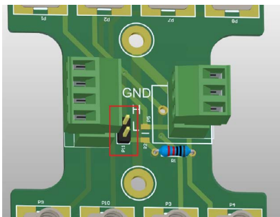
Fig. 61: Place for the jumper.
