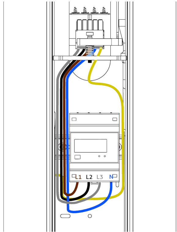
Fig. 46: Example of Enelion VERTICA Pole connection with the use of MID meter.
