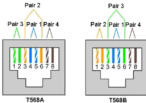
Fig. 52: Ending the Ethernet Patchcord according to TIA-568A/B do 100BaseT
