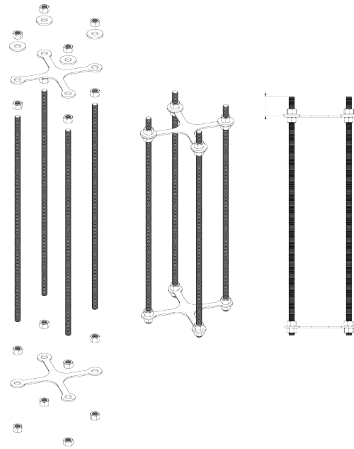
Fig. 28: Guidelines for the installation of the Enelion foundation set.
