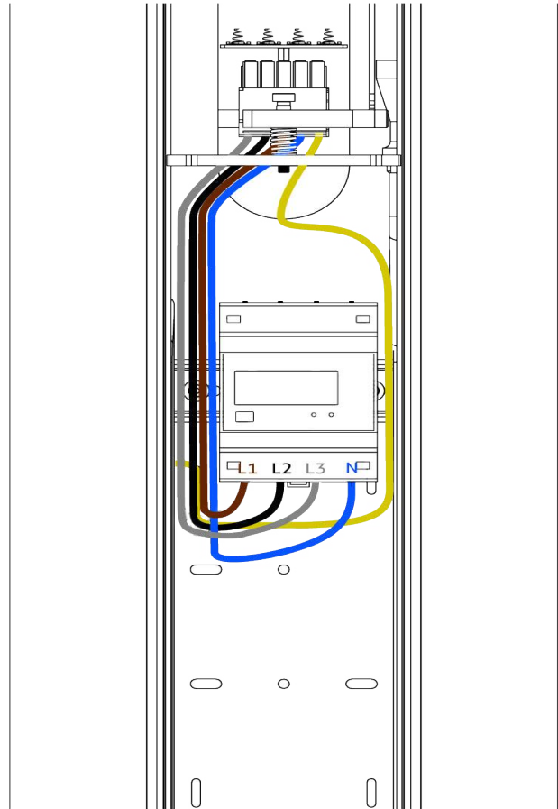
Fig. 43: MID meter fitted in Enelion VERTICA Pole.
