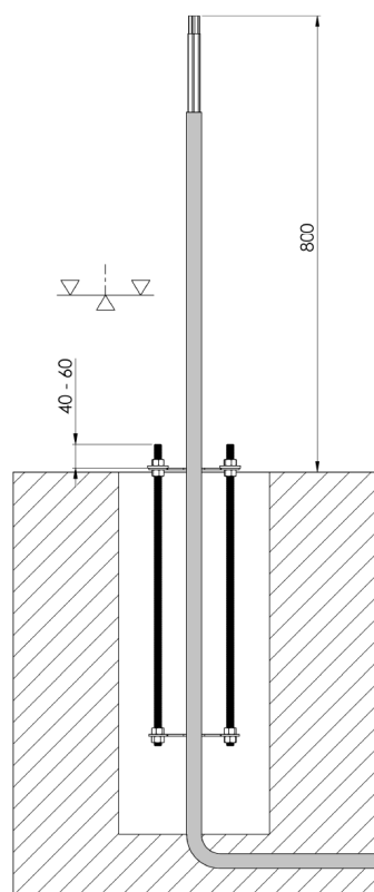
Fig. 29: Diagram of placing the foundation set in the excavation
