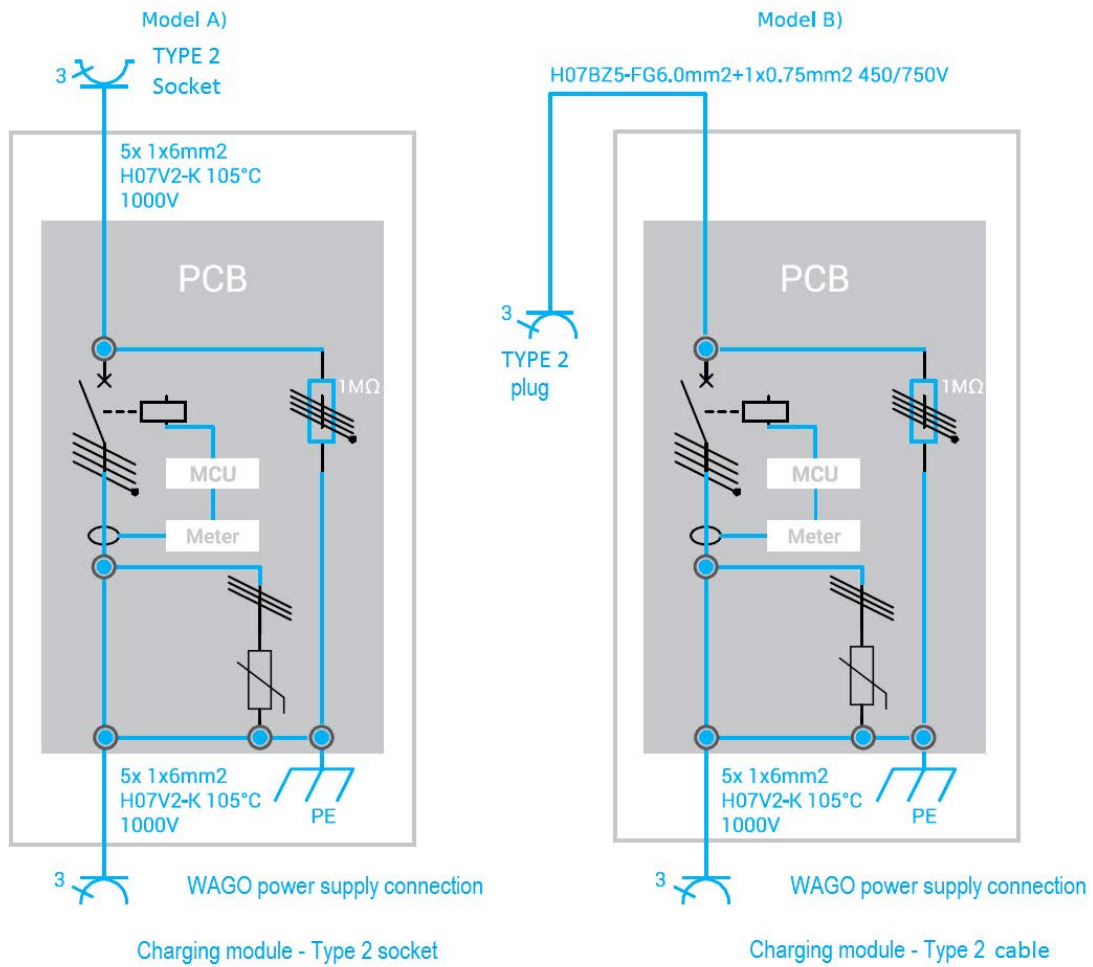
Fig. 19: Pictorial diagrams of Enelion VERTICA Modules part 1/2.
