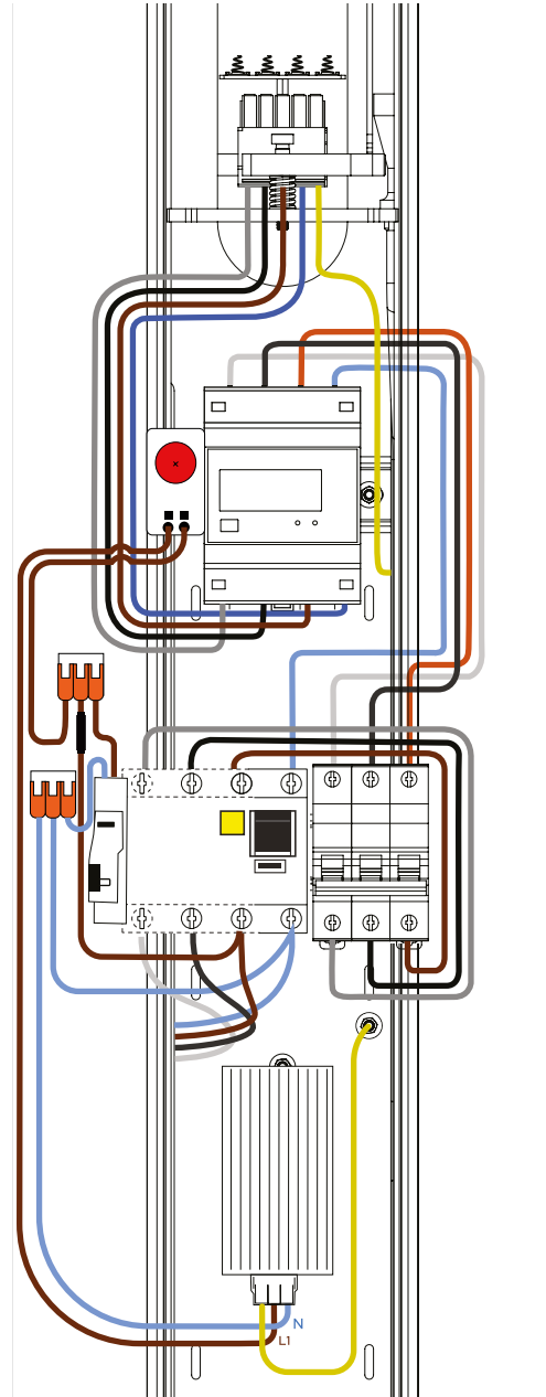
Fig. 51: Connecting the heating system in the ENELION VERTICA station on the opposite side of the pole.
