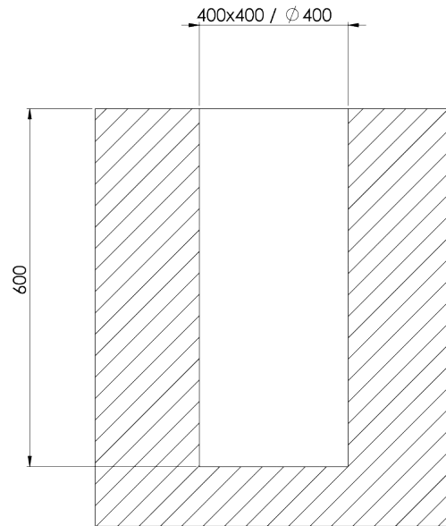
Fig. 22: Diagram of the foundation excavation.
