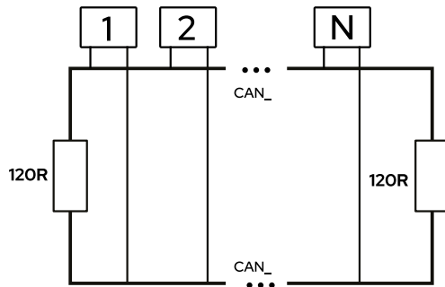
Fig. 59: Termination scheme of the communication bus.
