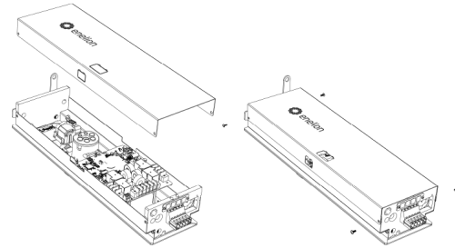
Fig. 76: Closing the Enelion VERTICA Module with RCMB.
