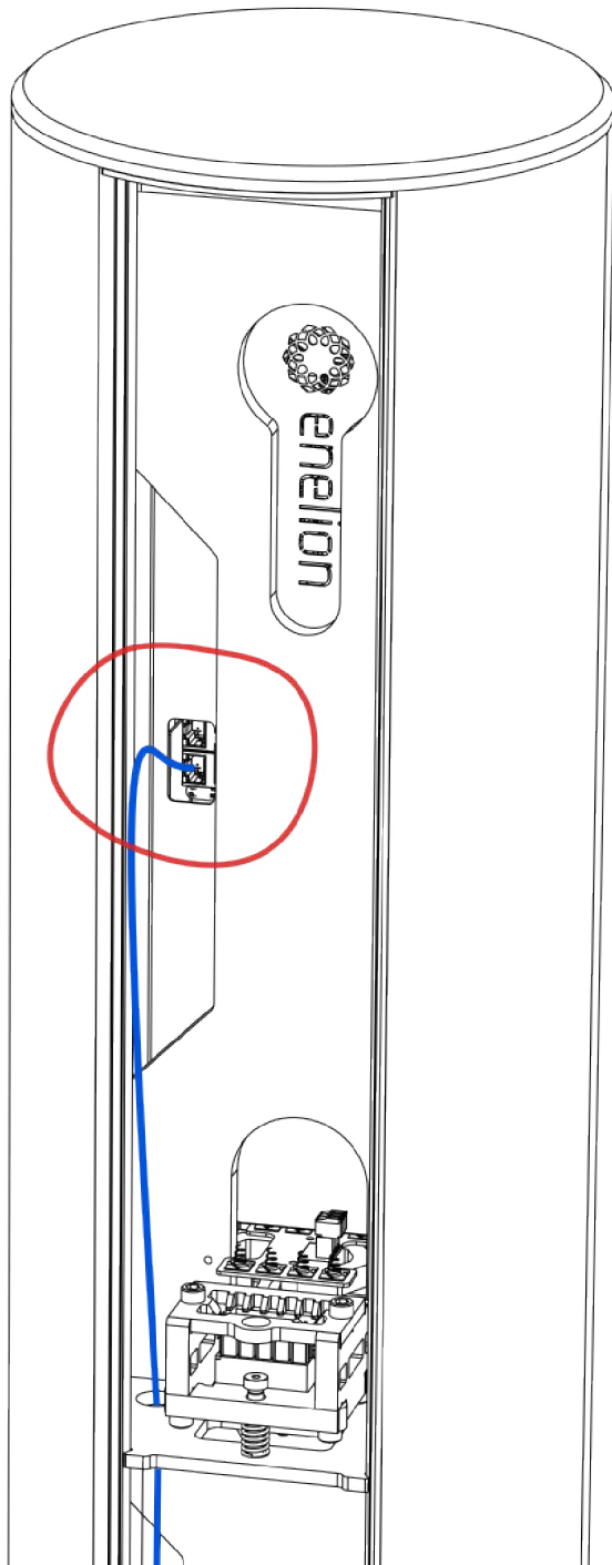
Fig. 55: Cable routed to the Ethernet socket.
