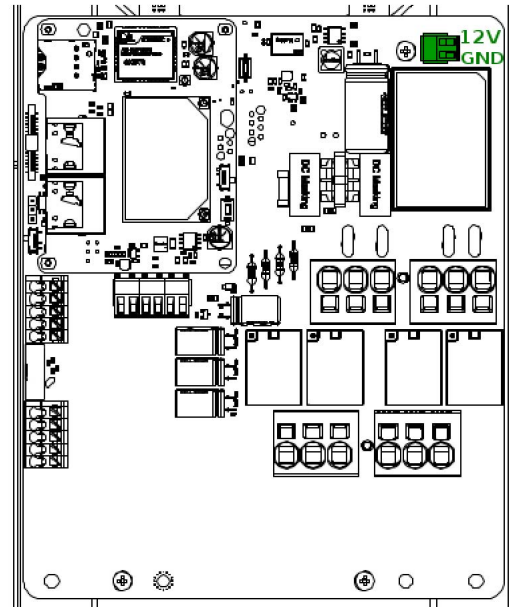
Fig. 79: Location of the power socket for LTE module power cable
