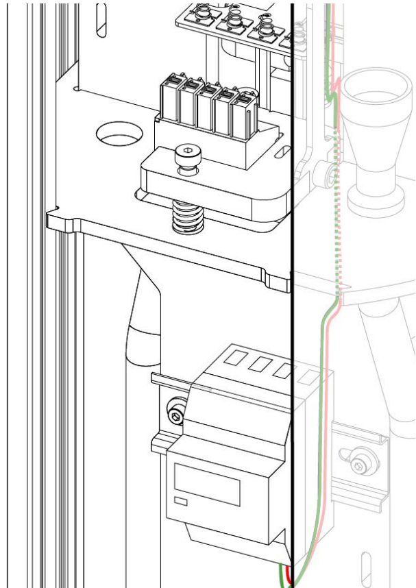
Fig. 62: Marking place in the pole for Enelion VERTICAN.
