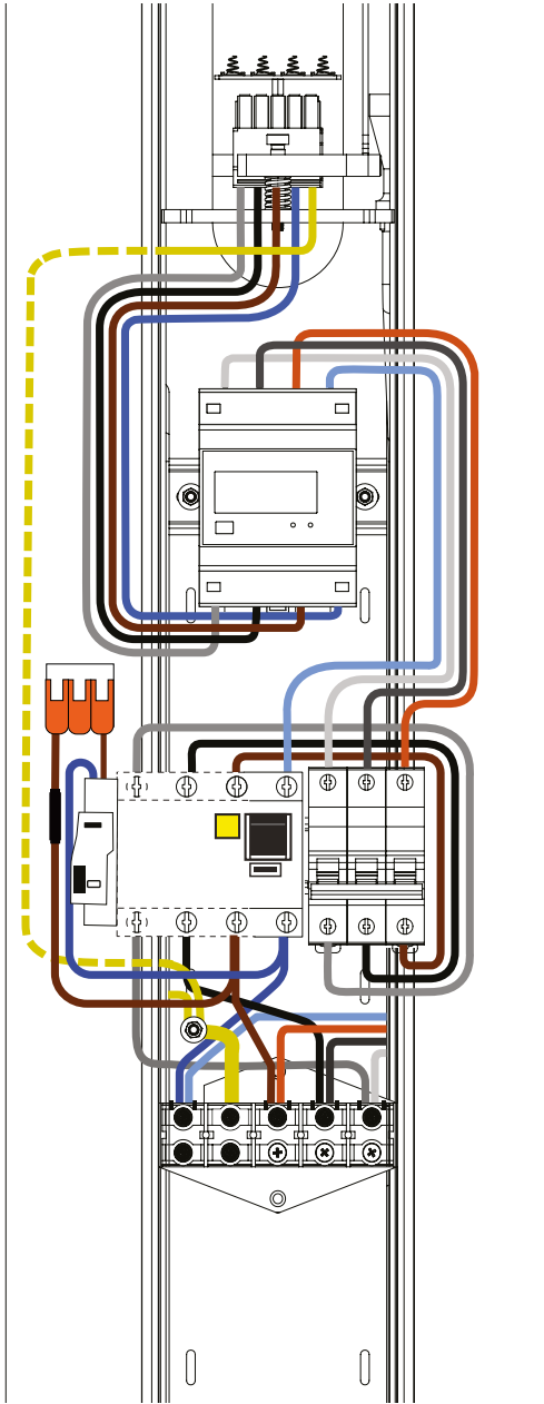
Fig. 50: Connecting the heating system in the ENELION VERTICA station
