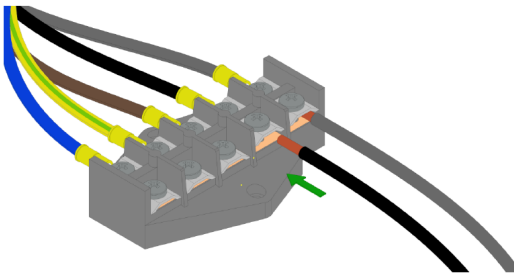
Fig. 25: Connection with solid conductors-wire
