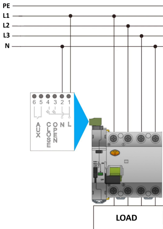
Fig. 11: Instructions for connecting RCD B with an automatic reclosing device to the power supply.
