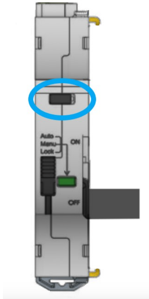
Fig. 12: Automatic reclosing device Interface
