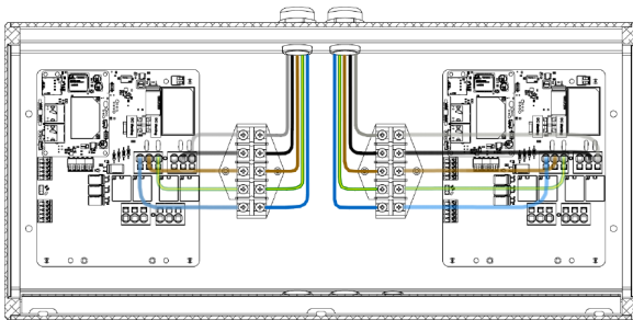
Fig. 26: Electrical connection executed correctly.
