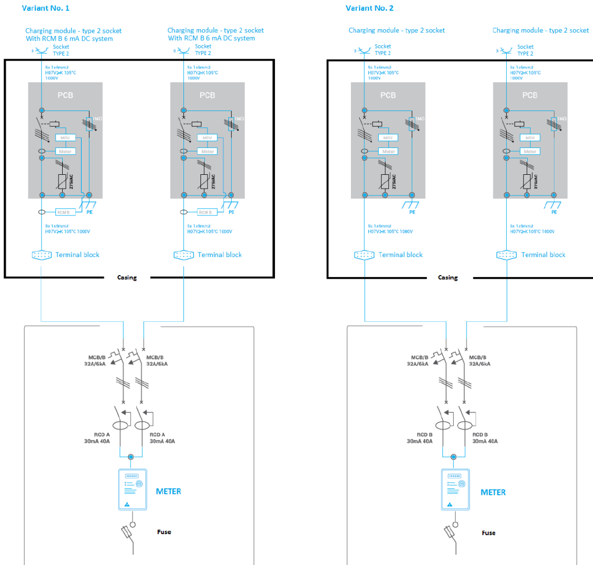
Fig. 22: Schemes of connection variants 1./2.
