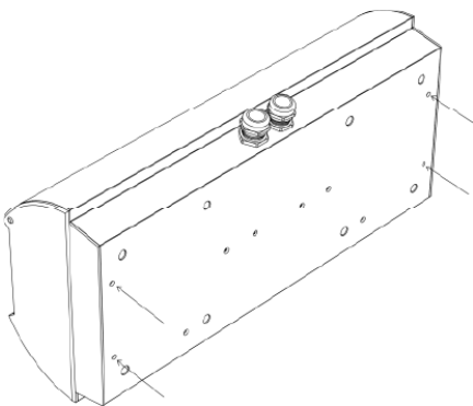
Fig. 17: Mounting holes of ENELION WALLBOX DUO POWER as seen from the back of the device.
