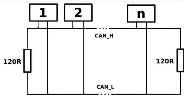
Fig. 34: Diagram of ENELION CHAIN communication cables connection (variant B)
