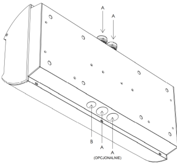
Fig. 20: Locations of cable entry points in ENELION WALLBOX DUO POWER.
