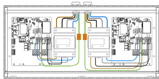
Fig. 27: Recommended connection when applying a MID meter.
