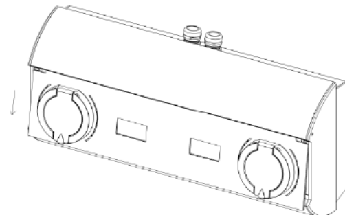
Fig. 8: Removing the front panel from the device housing.
