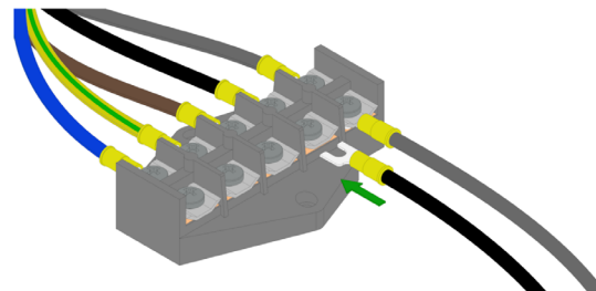
Fig. 24: Connection using fork terminals.
