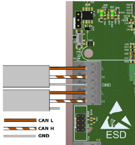
Fig. 34: Diagram of ENELION CHAIN communication cables connection (variant B)
