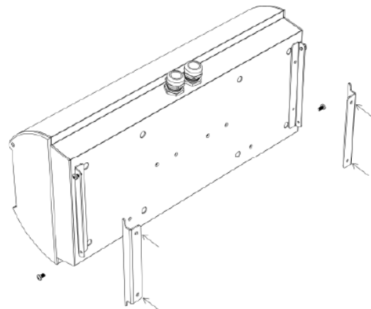
Fig. 16: Attaching the device to the holds with screws.
