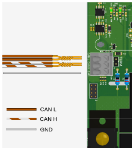
Fig. 33: Diagram of ENELION CHAIN communication cables connection (variant A)
