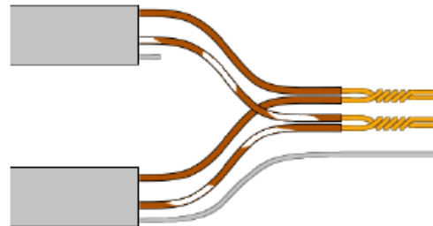
Fig. 31: Incoming and outgoing communication cable connection (variant A)
