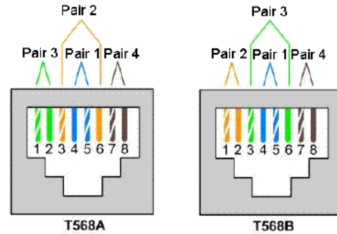
Fig. 40: Termination of the Ethernet cable according to TIA-568A/B to 100BaseT.
