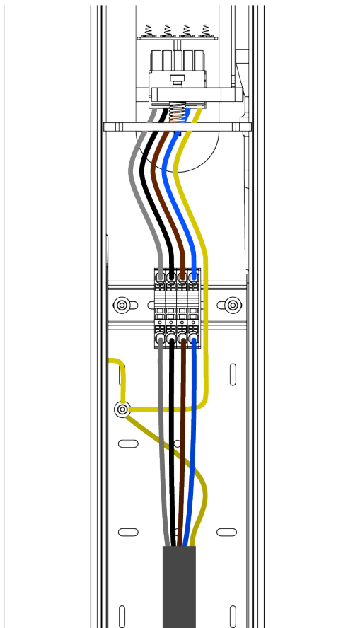
Fig. 38: Example Vertica Pole connection.
