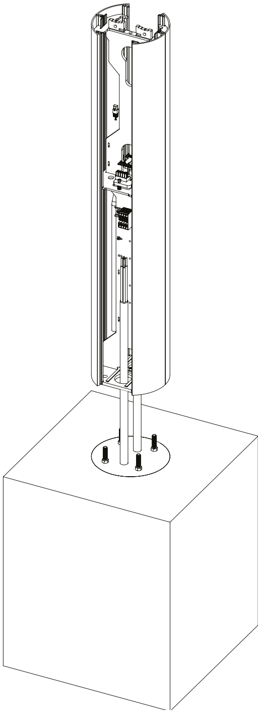
Fig. 36: Mounted and bolted Vertica Pole.
