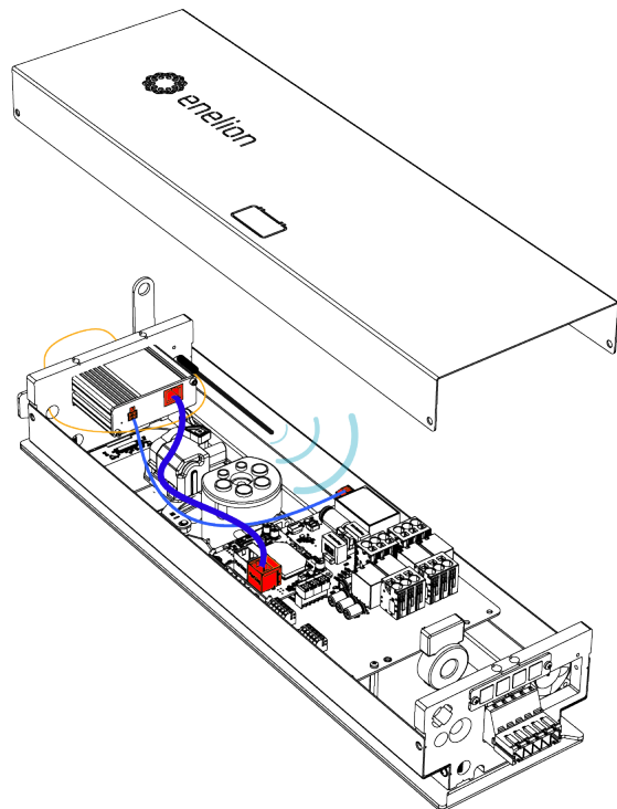
Fig. 73: Properly mounted LTE module.
