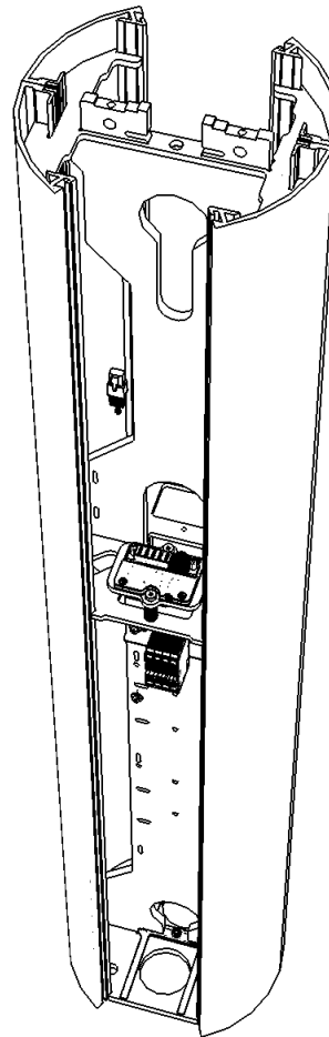
Fig. 10: Vertica pole equipped with Vertica link module
