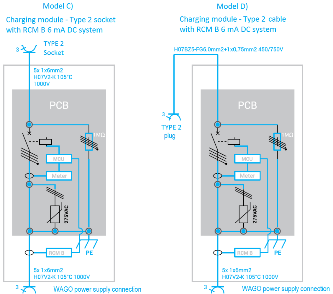
Fig. 17: Pictorial diagrams of Vertica Modules part 2/2.
