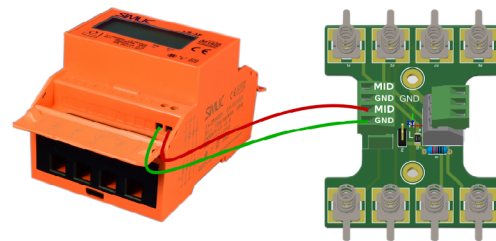
Fig. 44: Wiring diagram for MID meter communication wires for a Vertica pole equipped with a VertiCAN module.
