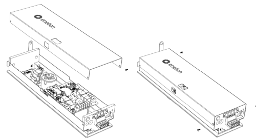
Fig. 61: Opening the Vertica Module.
