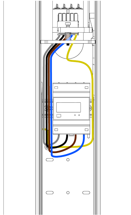
Fig. 43: Example of Vertica Pole connection with the use of MID meter.
