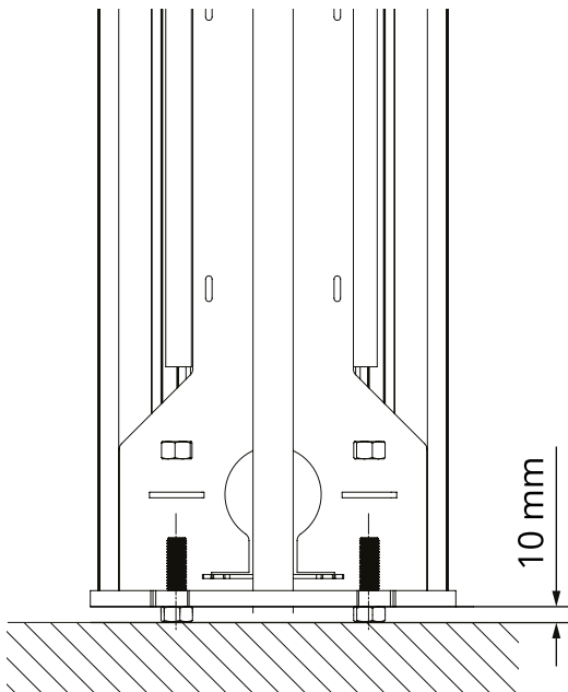
Fig. 35: Cross-section through the base of the Vertica Pole during assembly.
