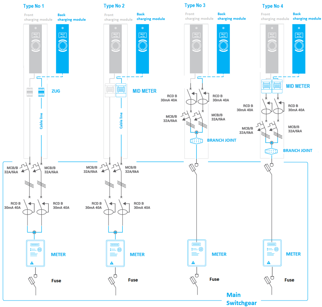
Fig. 14: Connection types part 1/2
