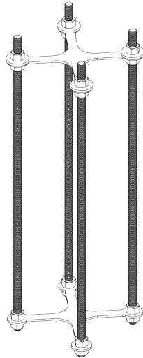
Fig. 24: Enelion foundation set.
