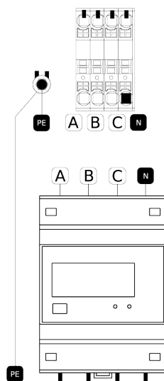
Fig. 42: Diagram of the relationship between standard connection and the one using a MID meter.
