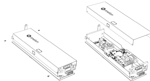
Fig. 65: Opening the Vertica Module.
