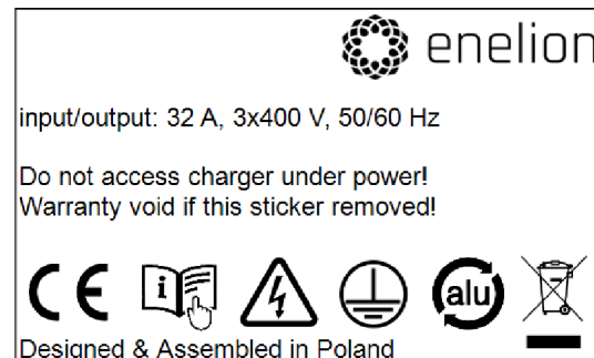
Fig. 1: Example of info plate
