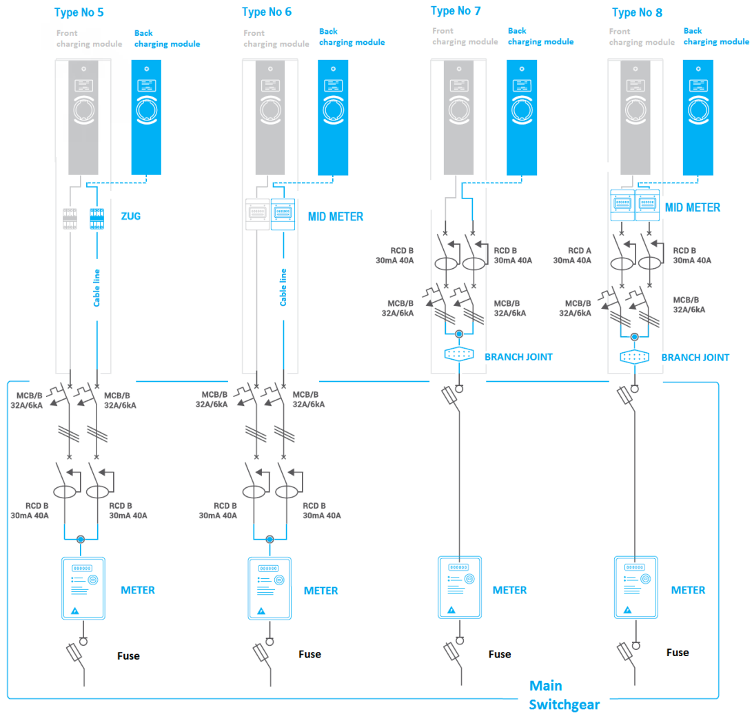
Fig. 15: Connection types part 2/2.
