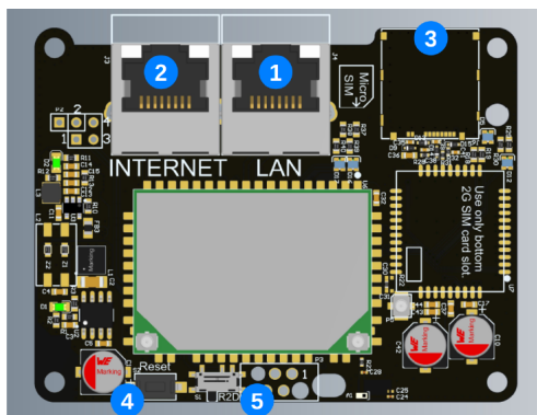
Fig. 56: The Enelion Bridge module
