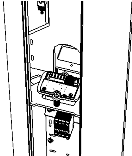
Fig. 53: CAN bus termination switch on the Vertica link module. To enable termination, set the switch to the "ON" position.
