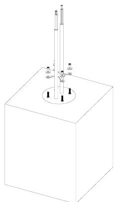
Fig. 31: Removing of the upper base plate from the foundation set.
