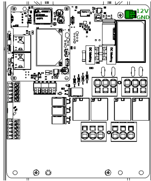
Fig. 72: Location of the power socket for LTE module power cable
