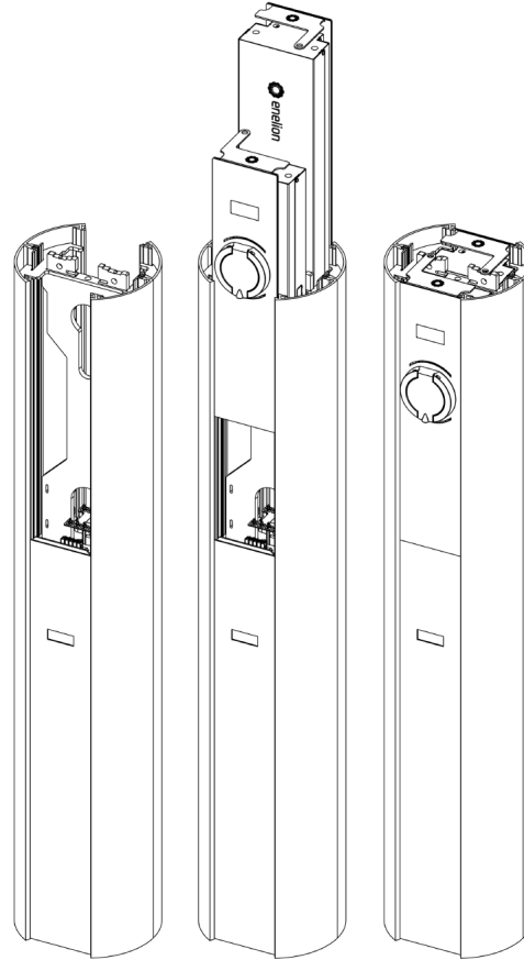
Fig. 13: Assembly of Vertica Modules
