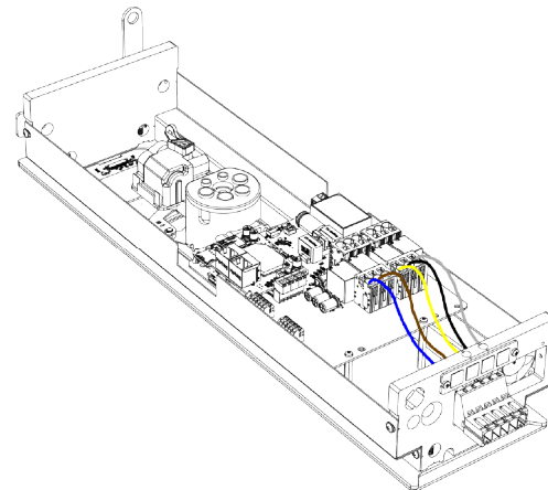
Fig. 66: The charging controller power connector on the Vertica Module.
