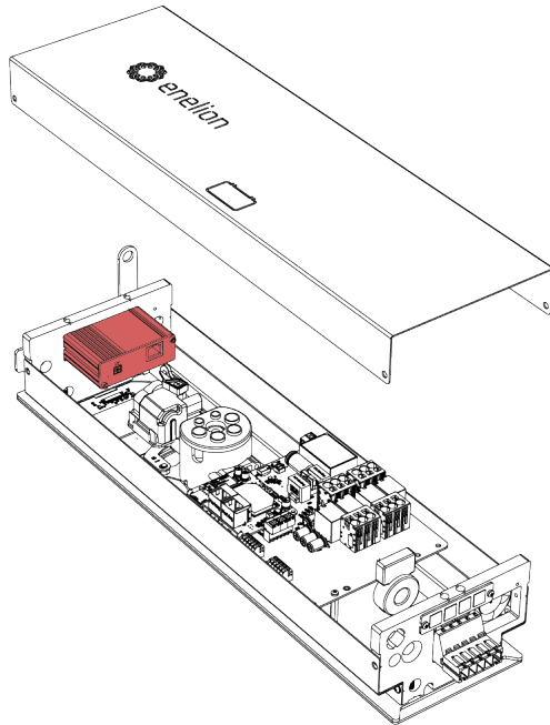
Fig. 71: Mounting the LTE module.
