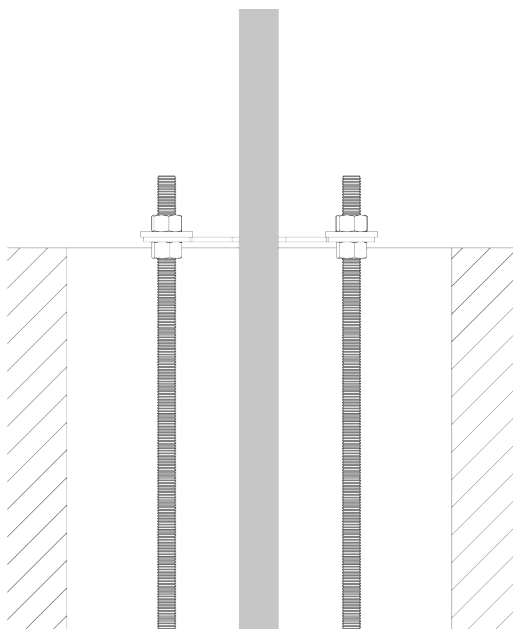
Fig. 27: Details of placing the upper base plate in the excavation
