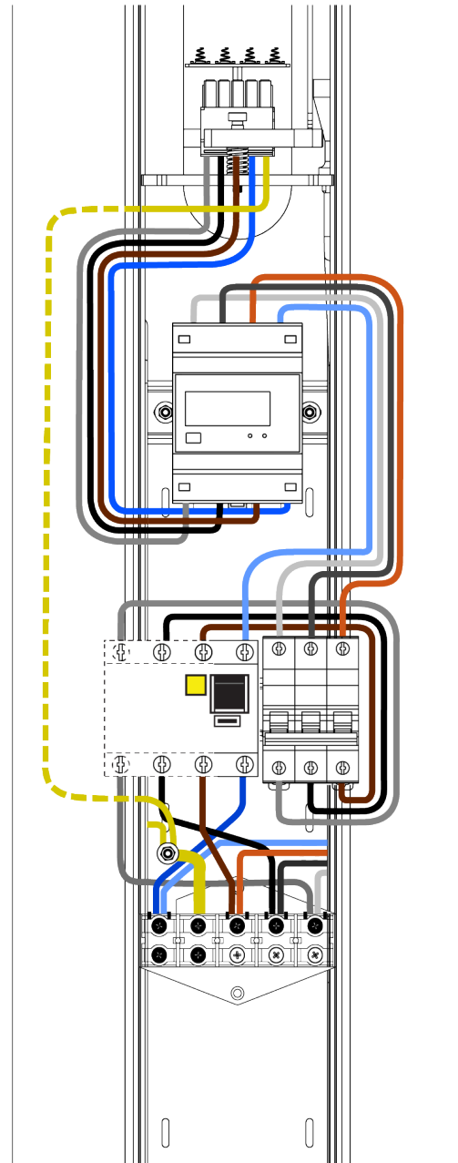
Fig. 58: Obverse of the Vertica Pole after mounting the Vertica Splitter with the MID meter present.
