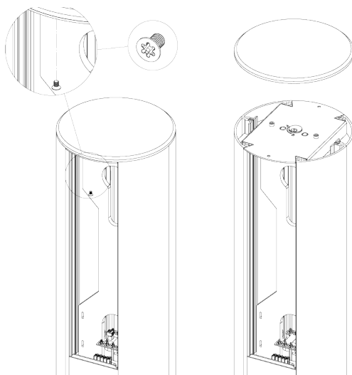
Fig. 4: Removing the cover of the Vertica Pole.
