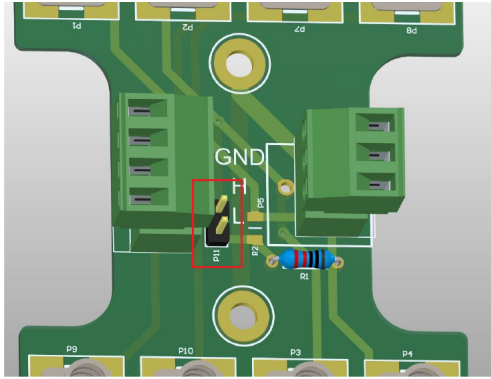
Fig. 50: Place for the jumper.
