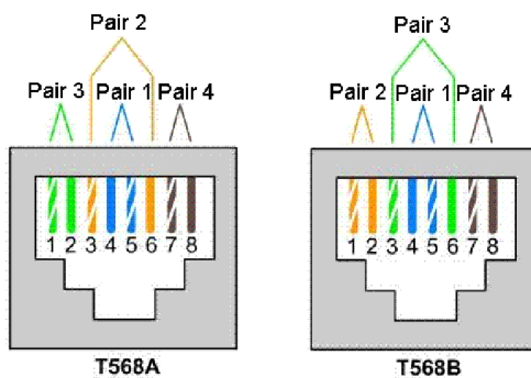
Fig. 54: Ending the Ethernet Patchcord according to TIA-568A/B do 100BaseT
