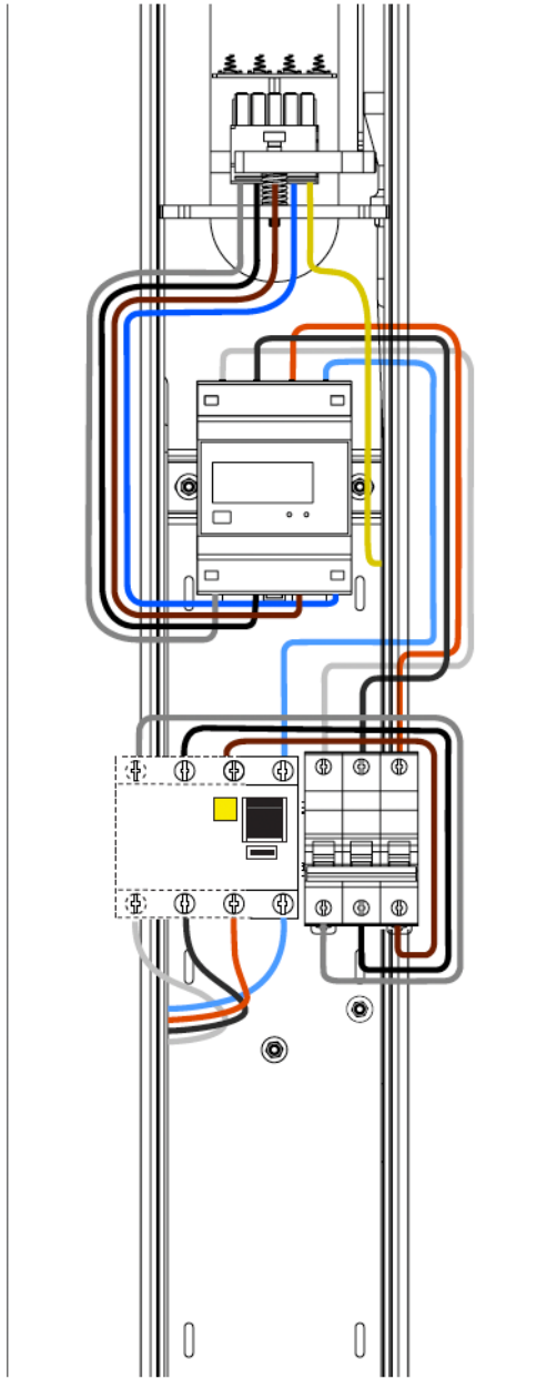
Fig. 59: Reverse of the Vertica Pole after mounting the Vertica Splitter with the MID meter present.
