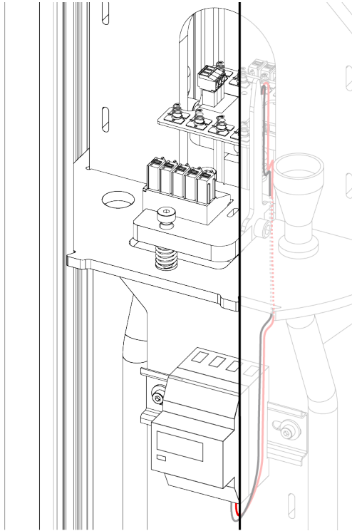
Fig. 41: Routing the MID meter signal cables.
