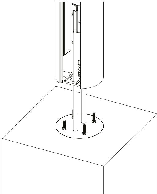
Fig. 34: Mounting Vertica Pole on the foundation.
