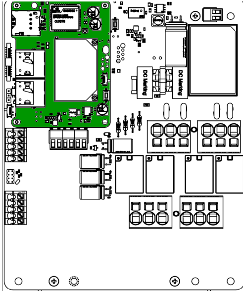
Fig. 63: Enelion Bridge attached to the Vertica Module.
