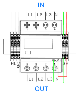
Fig. 45: Wiring diagram for MID meter communication wires for a Vertica pole equipped with a Vertica link module.
