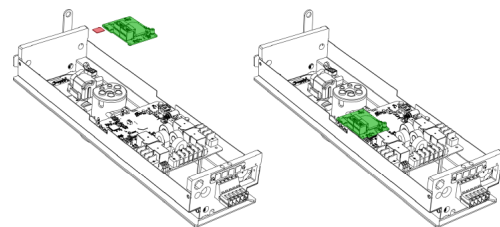
Fig. 62: Installing Enelion Bridge in the Vertica Module.
