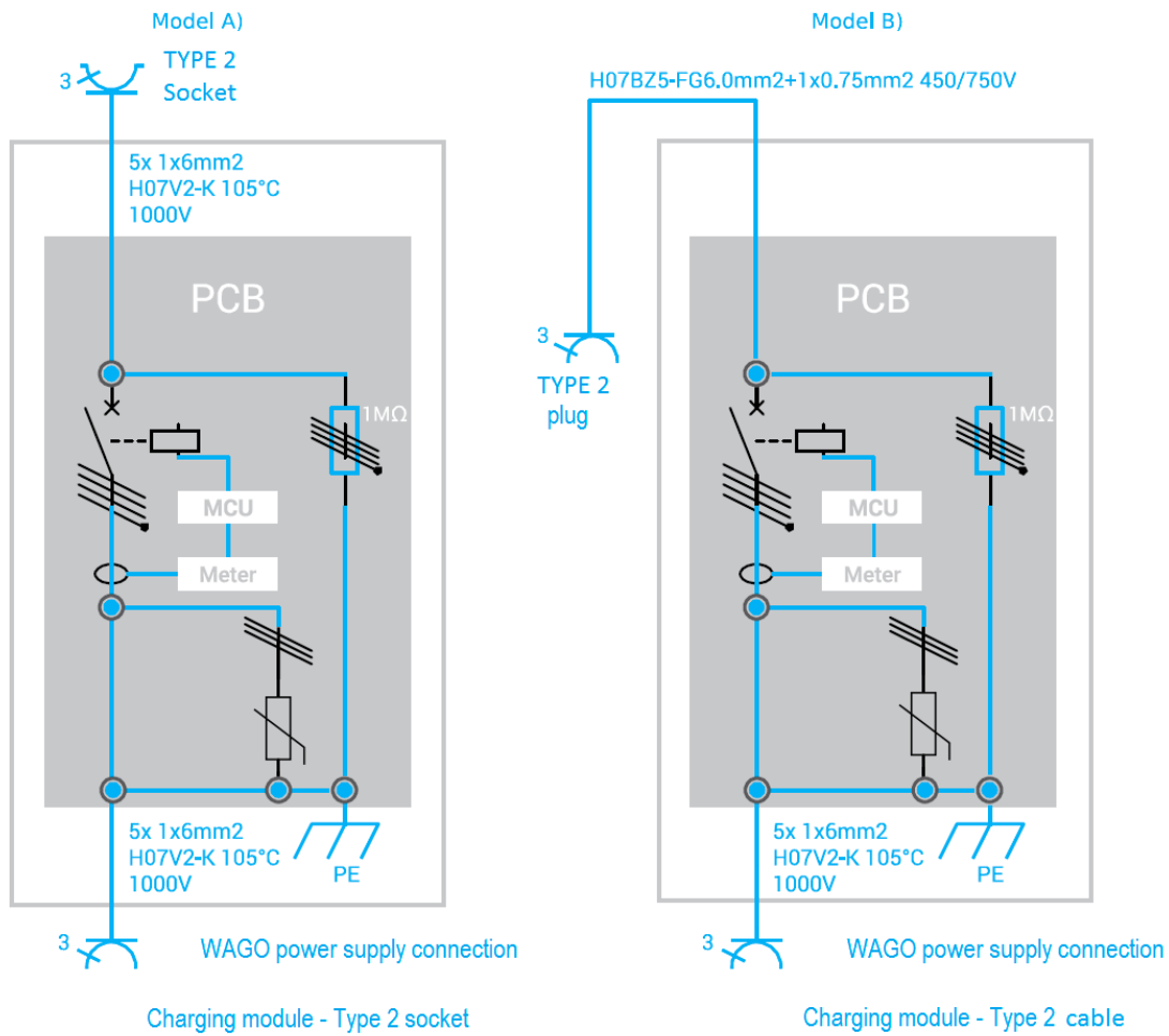
Fig. 16: Pictorial diagrams of Vertica Modules part 1/2.
