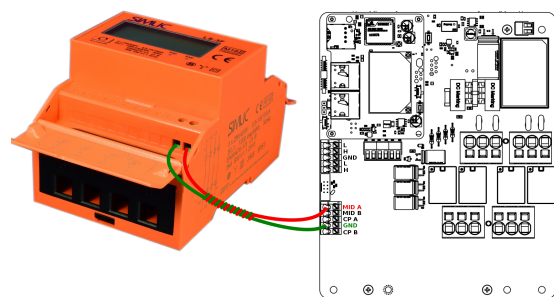
Fig. 22: MID meter communication connection.
