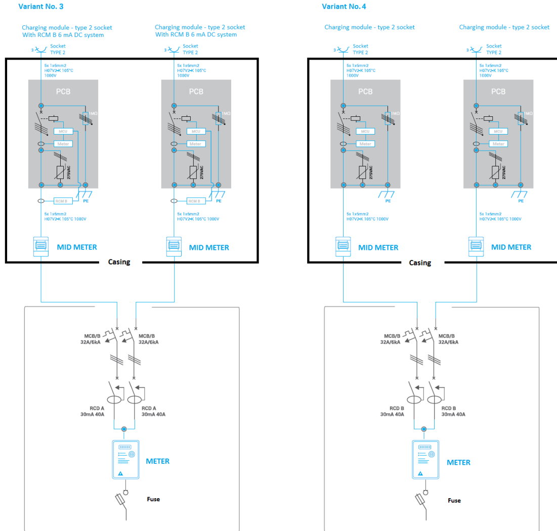
Fig. 20: Diagrams of connection types 2/2.
