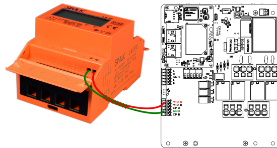
Fig. 25: MID meter communication connection diagram.
