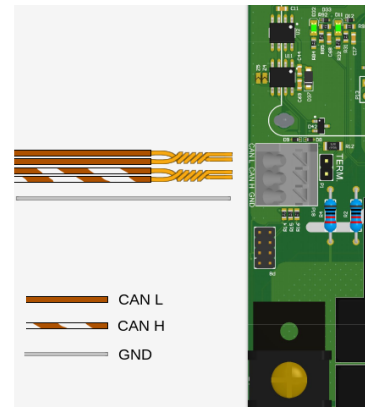
Fig. 22: Diagram of Enelion Chain communication cables connection (variant A)
