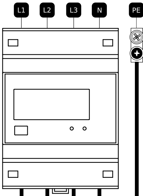
Fig. 17: Recommended connection when applying a MID meter.
