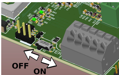
Fig. 27: The place of applying the terminating jumper (variant B)
