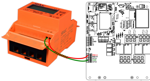
Fig. 16: MID meter communication connection.
