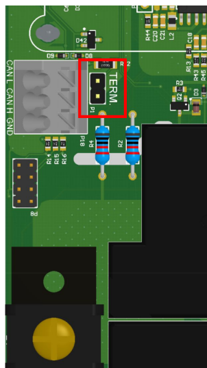
Fig. 26: The place of applying the terminating jumper (variant A)
