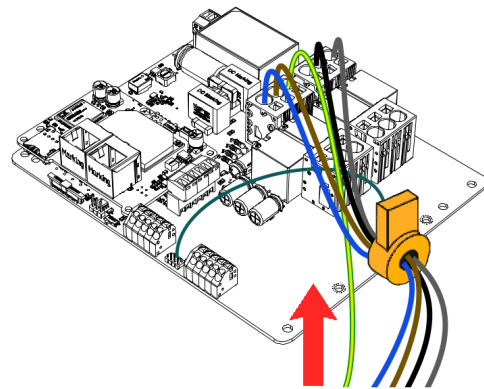
Fig. 19: RCM B connection
