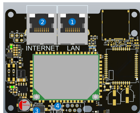
Fig. 29: Enelion Bridge module diagram.
