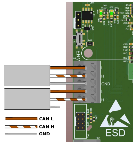
Fig. 23: Diagram of Enelion Chain communication cables connection (variant B)
