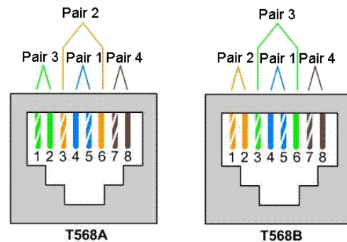
Fig. 28: Termination of the Ethernet cable according to TIA-568A/B to 100BaseT.
