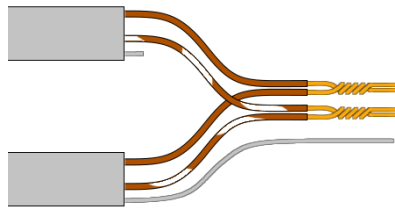
Fig. 20: Incoming and outgoing communication cable connection (variant A)
