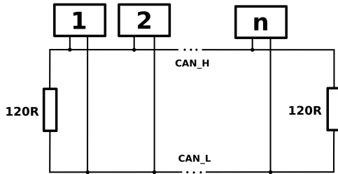
Fig. 24: Termination diagram.
