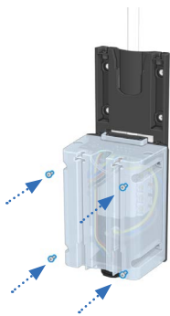
06 Mounting the cover with four screws
