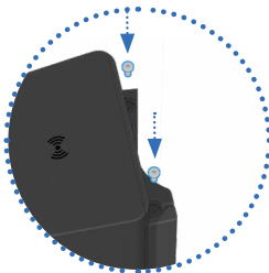
10 Tightening the head two bolts from above
