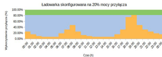
Fig. 11: No DLB system
