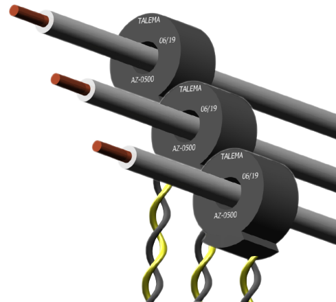
Fig. 2: Measuring coils in Home option
