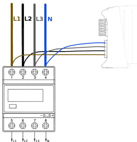
Fig. 8: Sample connection of the voltage lines to the selected apparatus in the switchboard.
